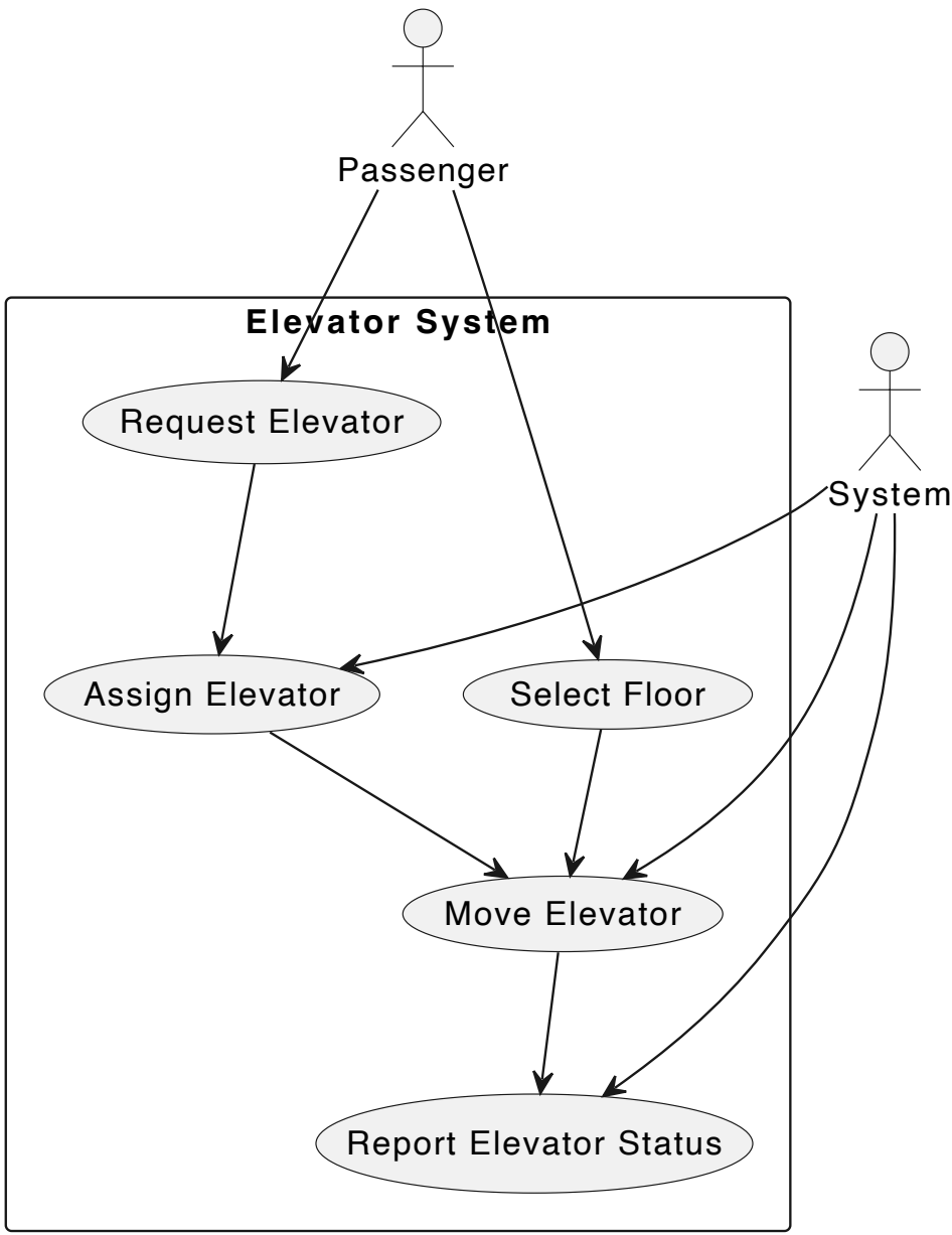
Use Case Diagram of Elevator Control System
