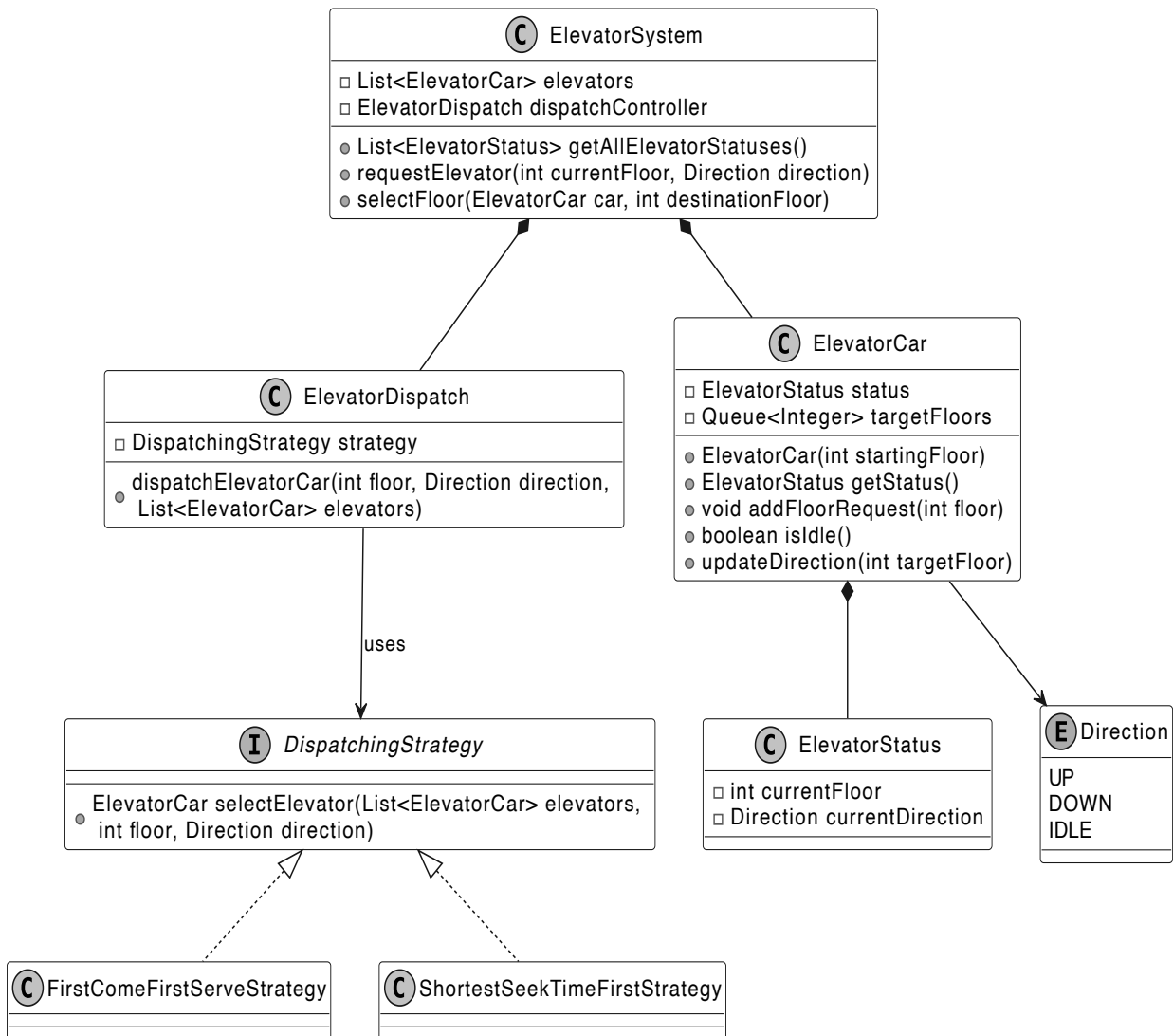
Class Diagram of Elevator System
